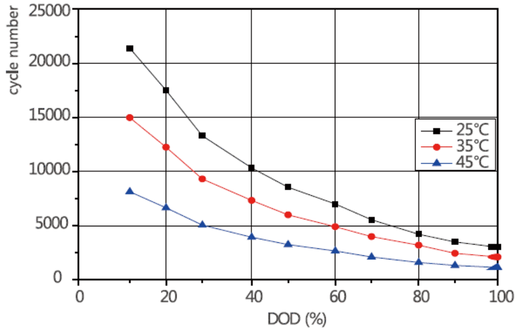
Cycle life curve under different DOD and temperature conditions for system
